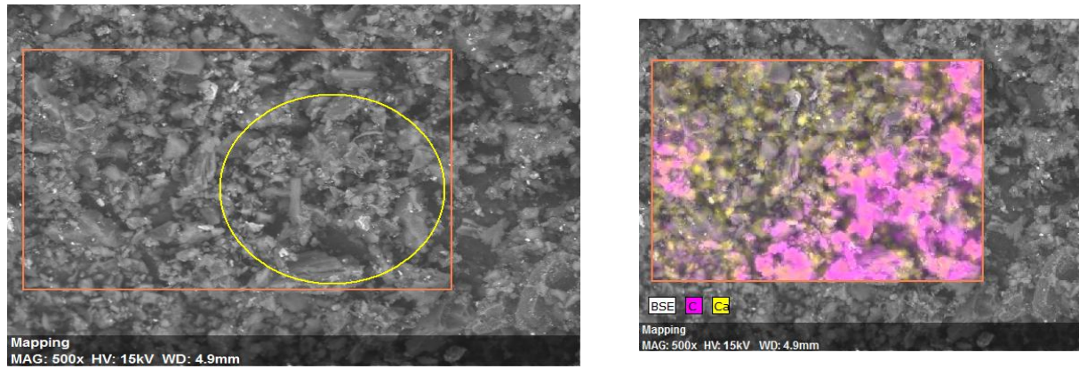
Fig. 1d The structural and surface characterization of activated carbon
