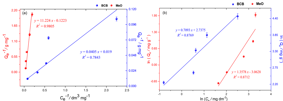
Figure 7. Linear fits of Langmuir (a) and Freundlich (b) isotherms and equilibrium data for BCB and MeO adsorption onto LPSH, experimental conditions: initial dye concentrations C_0 : 15 to 100 \text{mg dm}^{-3} (39 \mu\text{mol dm}^{-3} for BCB and 46 \mu\text{mol dm}^{-3} for MeO); W = 0.1 g for BCB and 0.2 g for MeO; pH 5 for BCB and pH 7 for MeO; contact time 20 min for BCB and 90 min for MeO; T = 298 K
