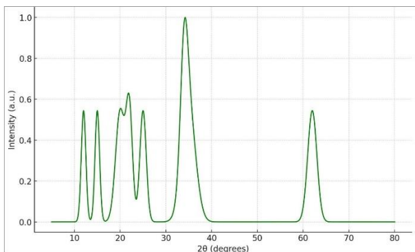
Figure 2. XRD pattern of sample.
