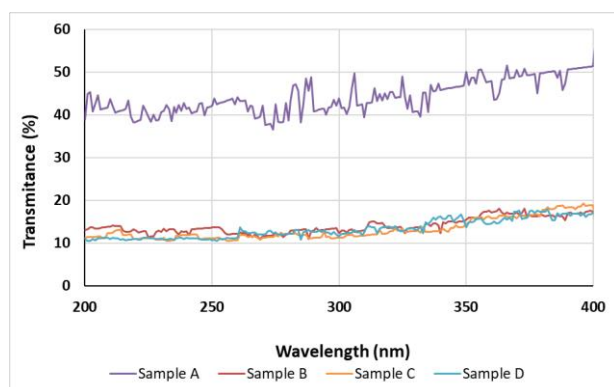
Figure 3. UV transmission diagram.
