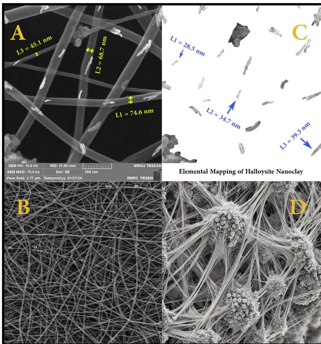
Figure 1. FESEM of: (A, B) Electrospun sample, (C) Elemental map, and (D) Frozen section.
