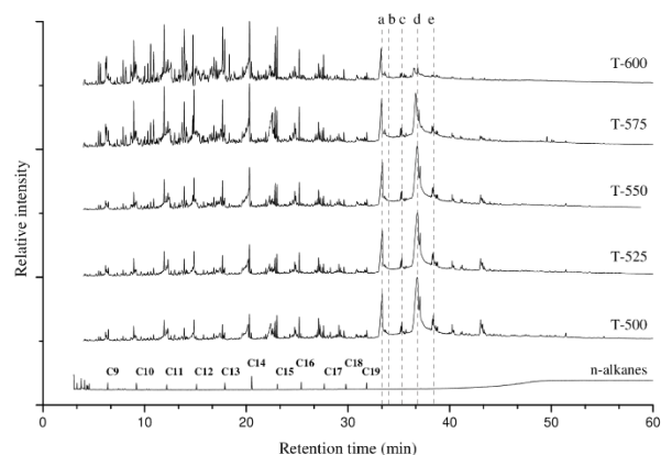
Figure 3. GC-MS profiles for n-alkane standard and bio-oil samples at T-500, T-525, T-550, T-575 and T-600. Peaks: (a) palmitic acid, (b) eicosanoic acid, (c) stearic acid, (d) oleic acid and (e) linoleic acid.
