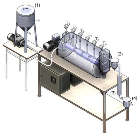
Figure 1. 3-D schematic view of the pyrolysis reactor. (1) - Feedstock reservoir; (2) - First bio-oil reservoir; (3) - Condenser; (4) - Second bio-oil reservoir.
