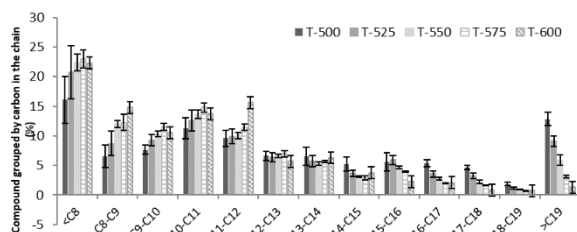
Figure 2. Distribution of compounds in bio-oils according to carbon number.
