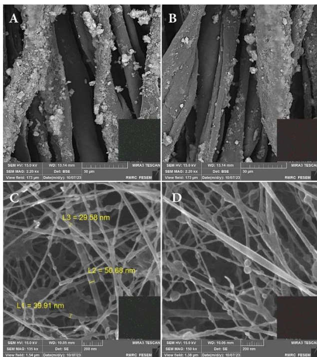
Figure 1. SEM of samples and elemental mapping of Sr and Zn.
