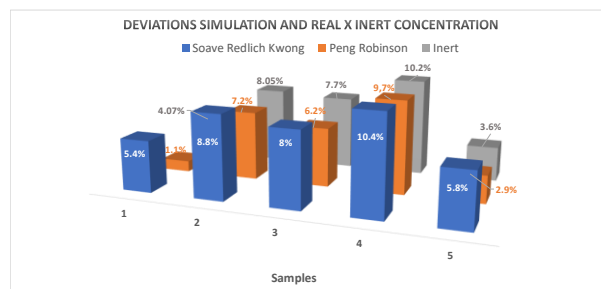
Figure 3. Deviations between the simulation results and actual plant data.
