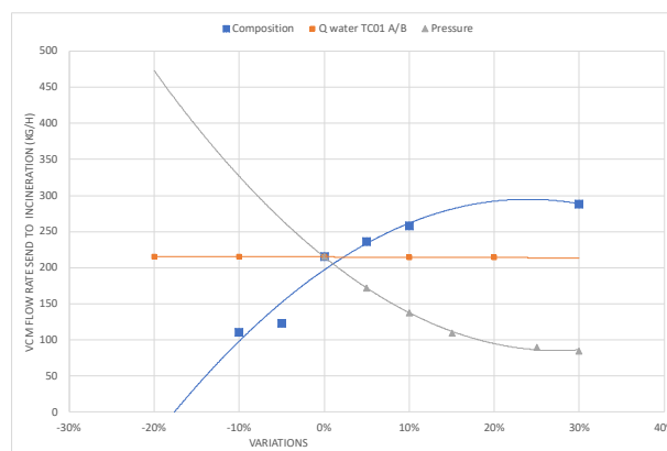
Figure 4. VCM flow rate to incineration after process changes.
