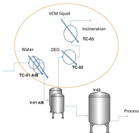
Figure 1. VCM recovery unit heat exchange system.
