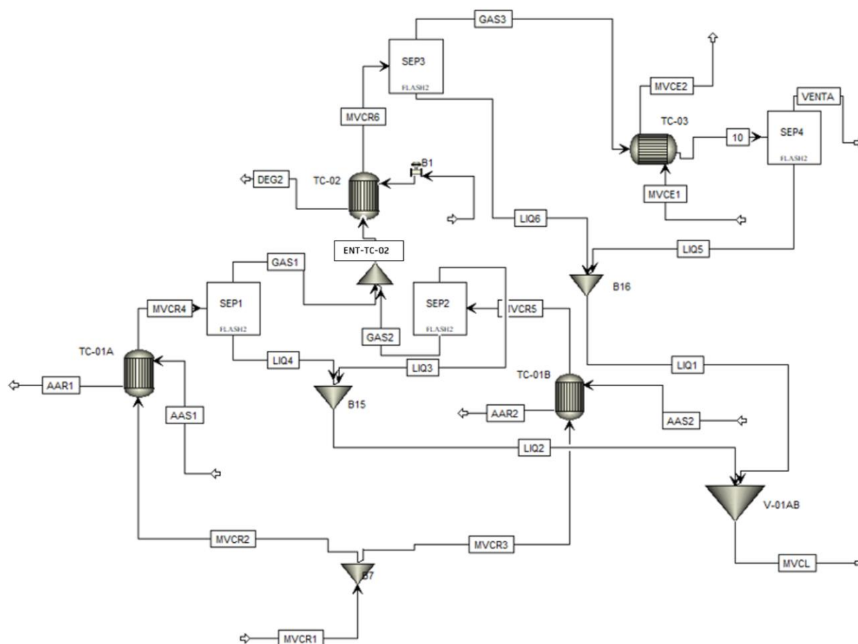
Figure 2. VCM recovery unit flowchart for process simulation.
