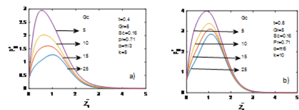
Figure 4. Velocity profiles for different values of 'Gc': (a) \alpha=n/3 , k=5 , t=0.4 , Pr=0.71 , Sc=0.16 , Gr=5 ; (b) \alpha=n/6 , k=10 , t=0.6 , Pr=0.71 , Sc=0.16 , Gr=5 .
