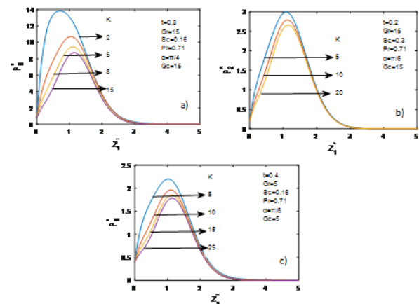
Figure 3. Velocity profiles for different values of 'K': (a) \alpha=n/4 , t=0.8 , Pr=0.71 , Sc=0.16 , Gr=15 , Gc=15 ; (b) \alpha=n/6 , t=0.2 , Pr=0.71 , Sc=0.3 , Gr=15 , Gc=15 ; (c) \alpha=n/6 , t=0.4 , Pr=0.71 , Sc=0.16 , Gr=5 , Gc=5 .
